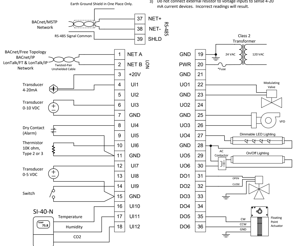
This diagram is an example of device connections and no reference to an application is being provided.
